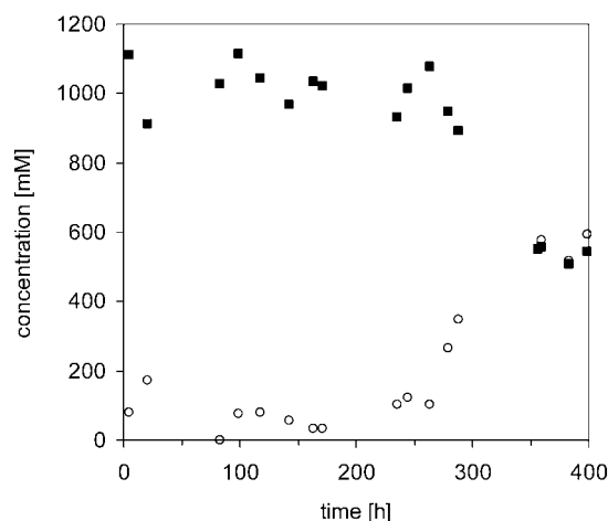
Figure 7. Time course for conversion of 1.13 M acrylonitrile in a column reactor containing 3 mm diameter catalyst beads (cell lot A) at 5 °C: acrylamide (■), acrylonitrile (○). Flow rate adjusted to maintain >90% conversion: 0–21 h at 0.5 mL/min, 21–118 h at 0.4 mL/min, 118–143 h at 0.35 mL/min, 143–399 h at 0.3 mL/min. Catalyst productivity from 0–263 h was 155 g acrylamide/g dcw.
