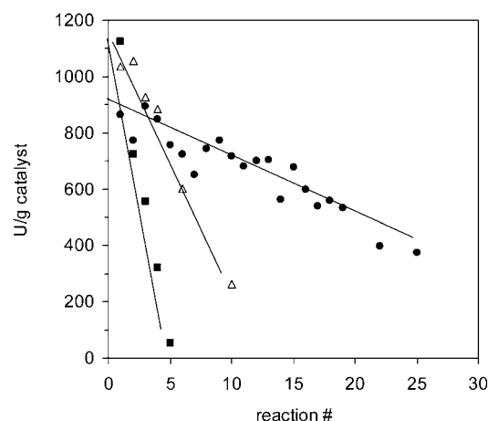
Figure 3. Effect of acrylonitrile concentration on recovered NHase activity of alginate-immobilized E. coli SW132 in consecutive batch recycle reactions at 35 °C; acrylonitrile: 1.06 M (●), 2.05 M (△), 3.04 M (■).
