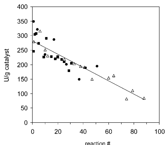
Figure 5. Specific activity of alginate-immobilized E. coli SW132 (1-mm diameter catalyst beads) in consecutive 1.06 M acrylonitrile batch reactions with catalyst recycle at 5 °C: no added acrylamide (■), 1.4 M added acrylamide (△, trend line), 2.9 M acrylamide (●).
