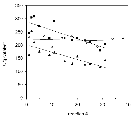
Figure 6. Comparison of recovered activity of 1-mm and 3-mm bead diameter immobilized cell catalysts in consecutive 1.06 M acrylonitrile batch reactions with catalyst recycle at 5 °C: 1 mm diameter, cell lot B (■), 3 mm diameter, cell lot B (▲), 3 mm diameter, cell lot A (○).
